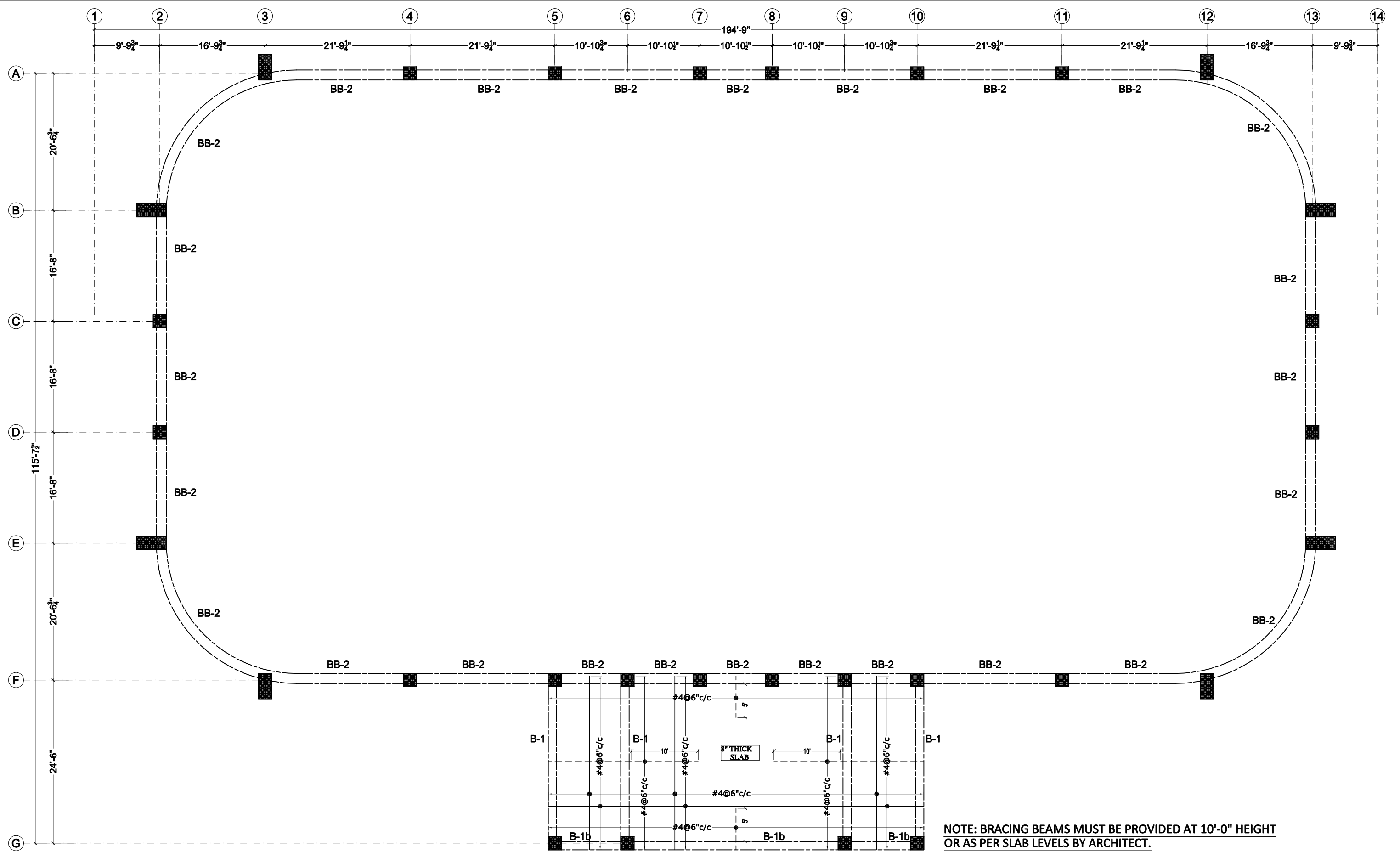
TOP ROOF BEAMS KEY PLAN
