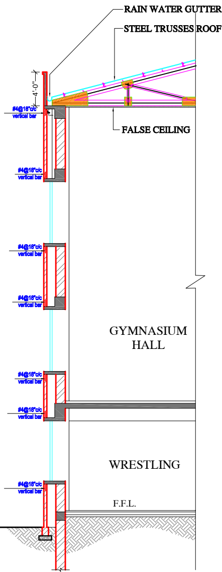
WALL SECTION-X
